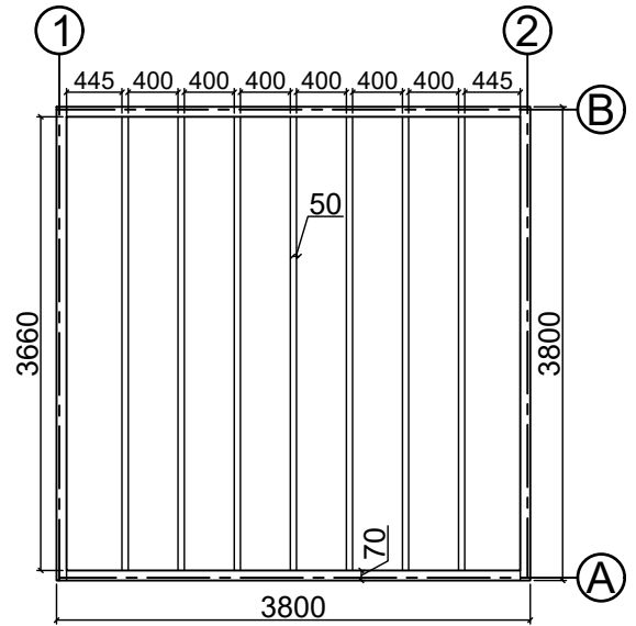
Base plan
