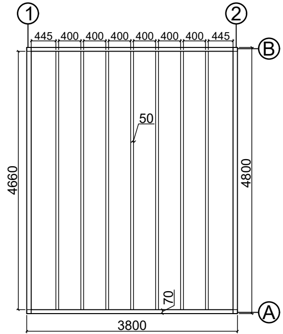
Base plan
