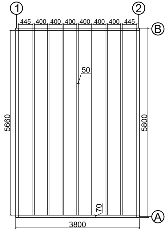
Base plan
