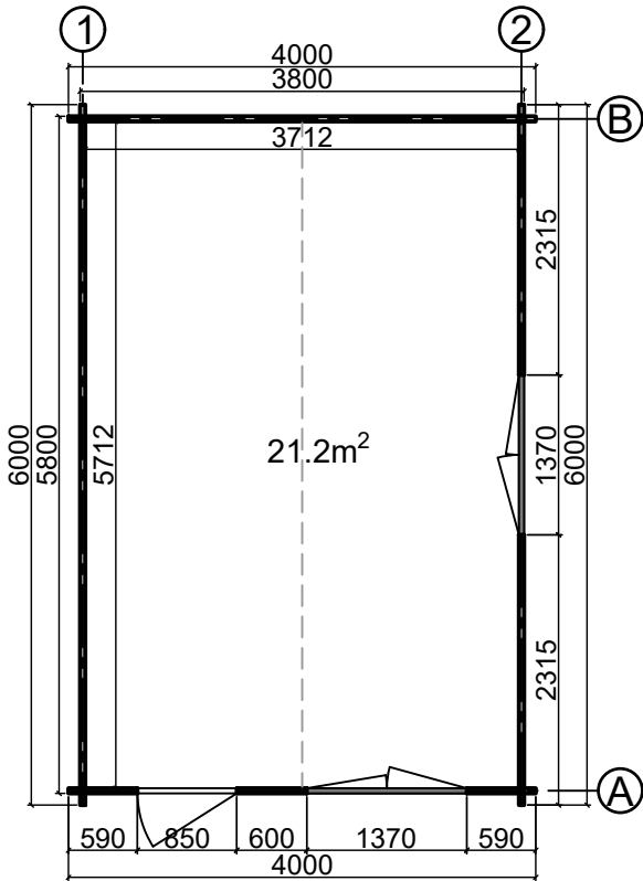
Floor plan
