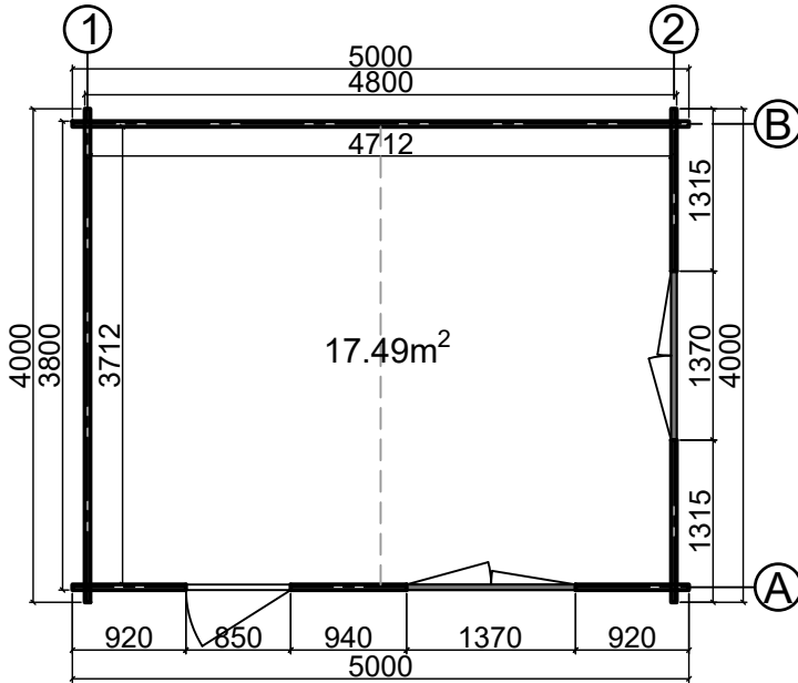
Floor plan
