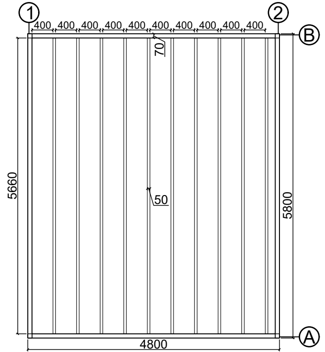
Base plan
