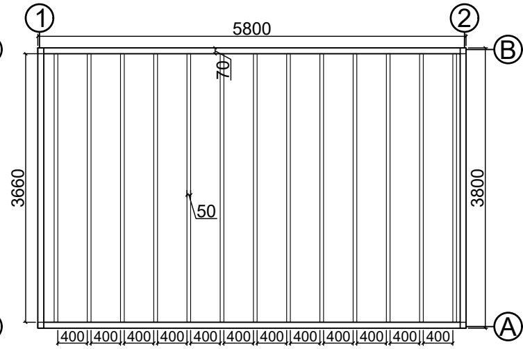
Base plan
