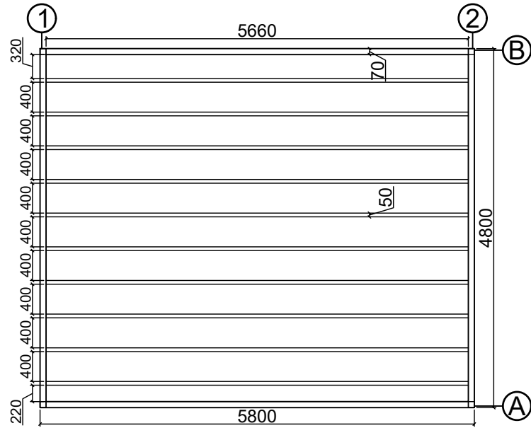
Base plan
