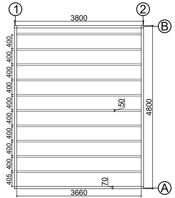
Base plan
