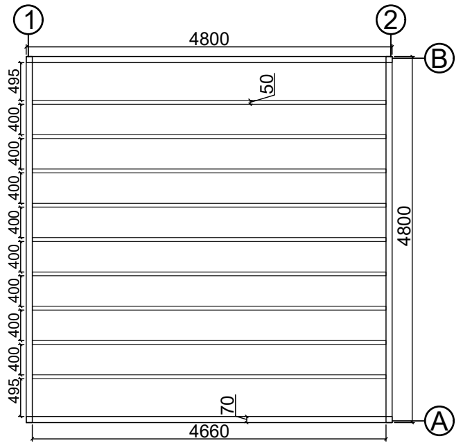
Base plan
