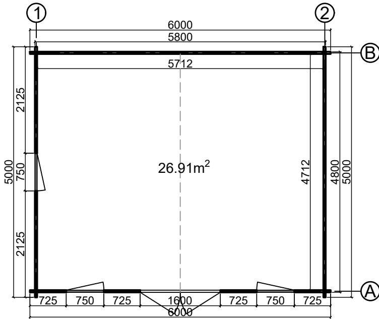
Floor plan
