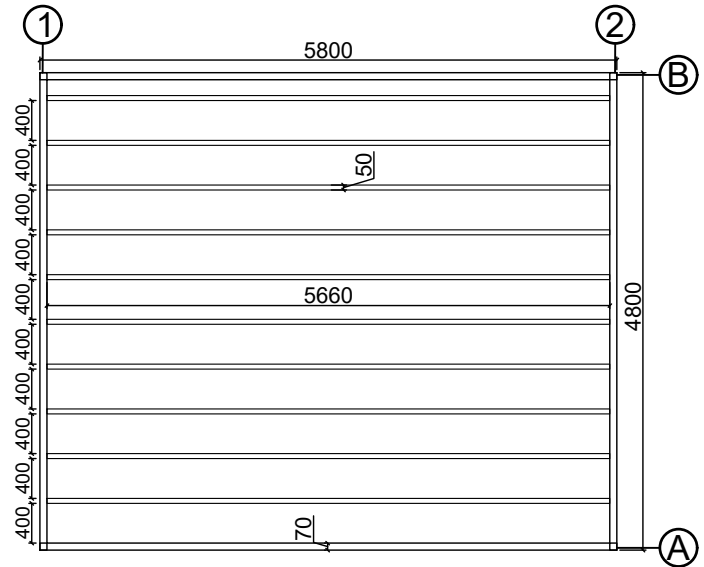
Base plan
