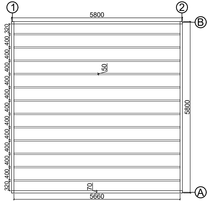
Base plan
