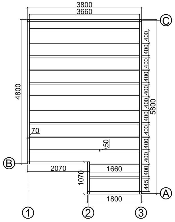
Base plan
