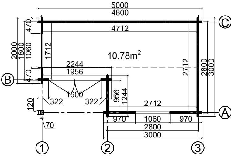
Floor plan
