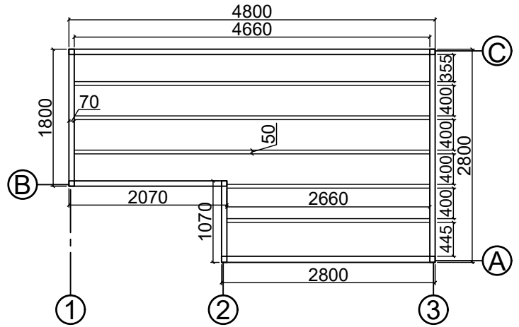
Base plan
