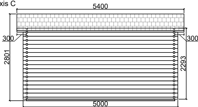
Axis C
