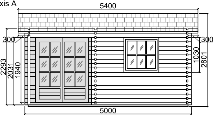
Axis A
