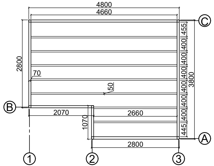
Base plan
