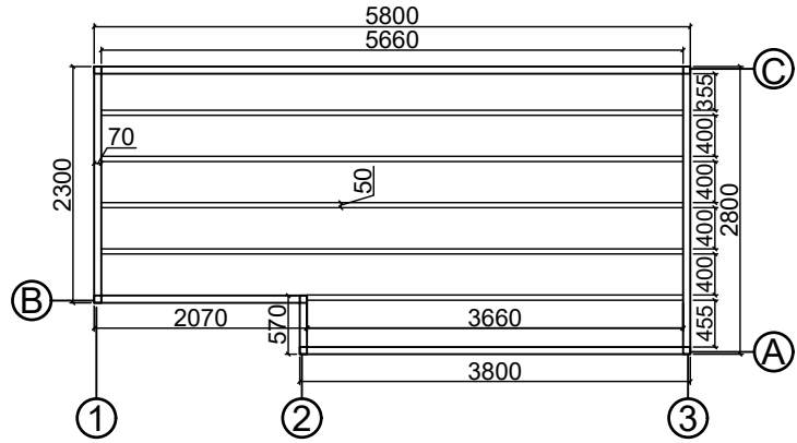
Base plan
