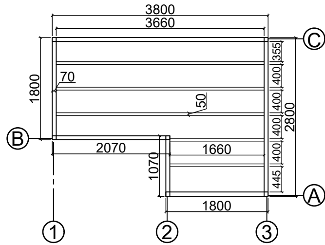
Base plan
