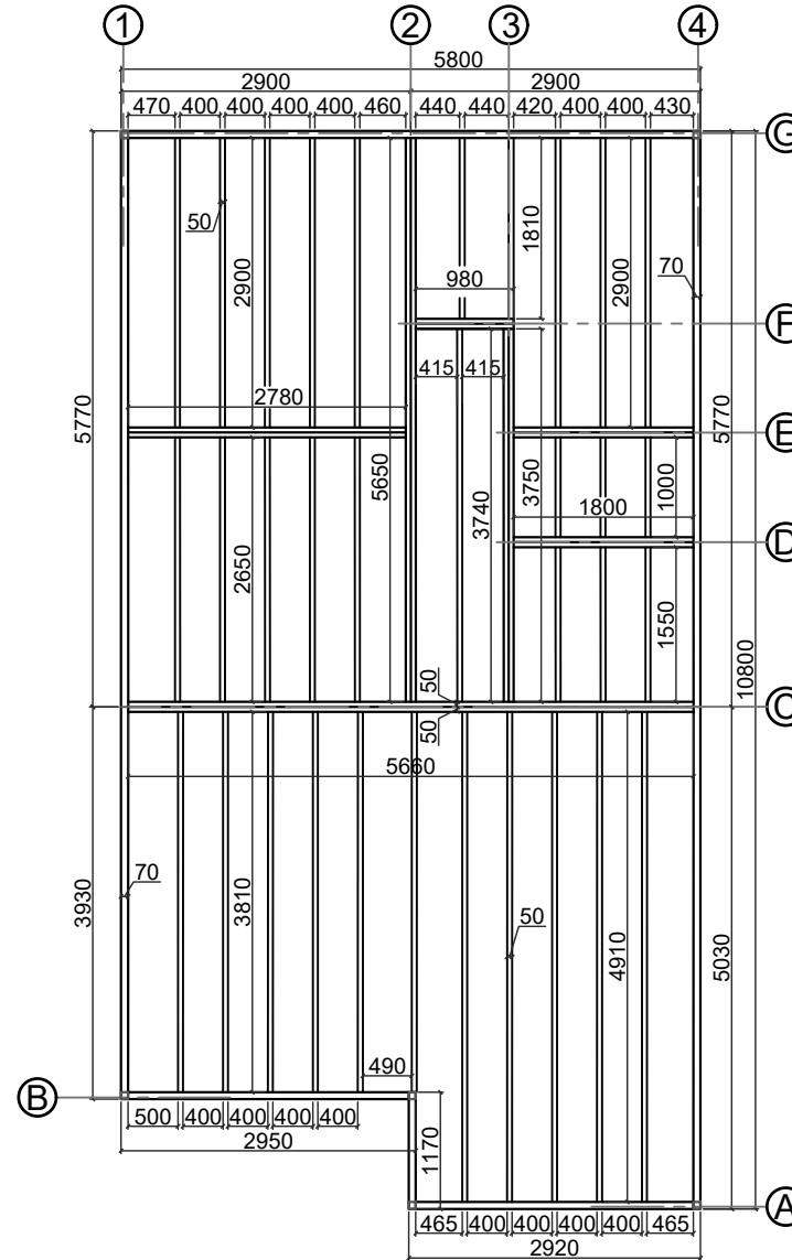
Base plan
