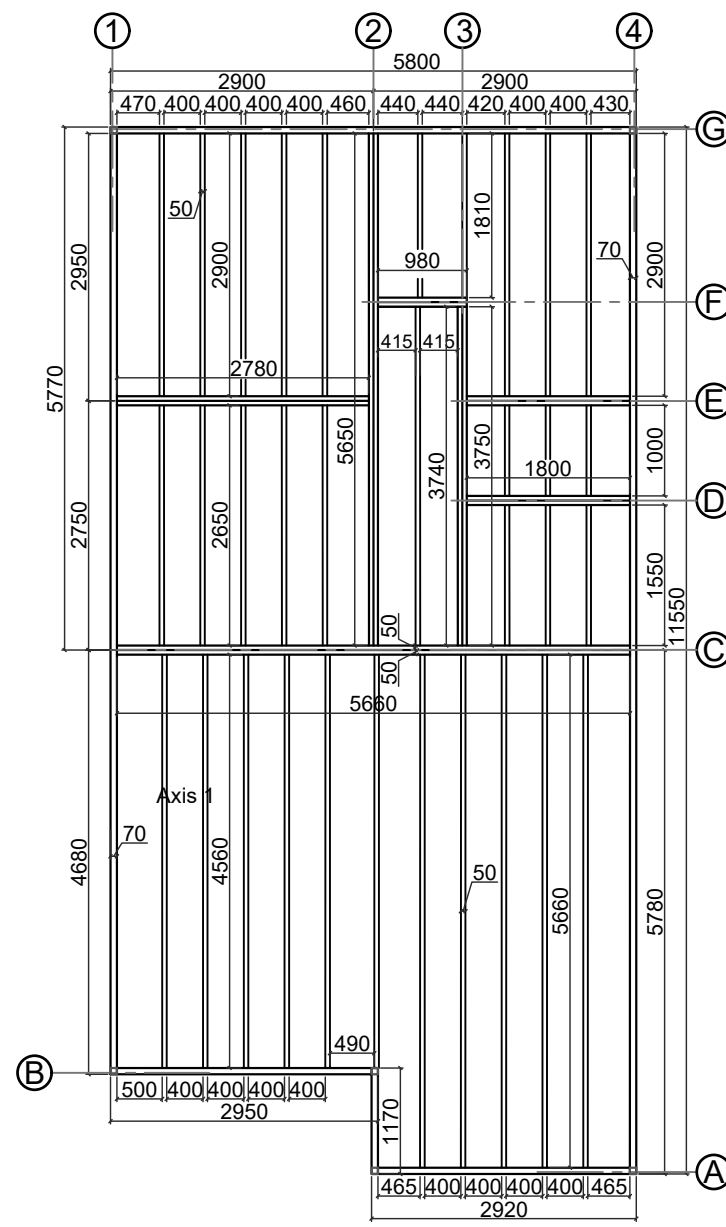
Base plan
