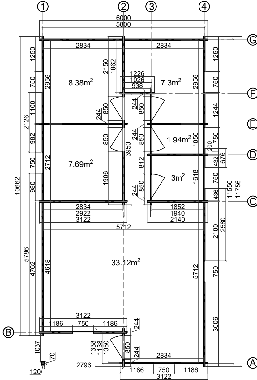
Floor plan
