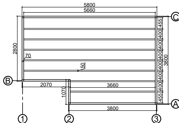
Base plan
