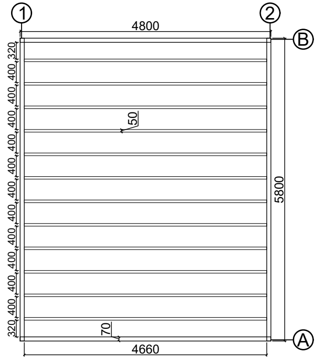
Base plan
