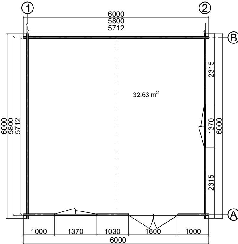
Floor plan
