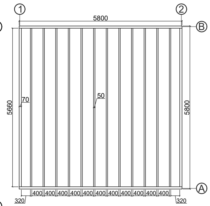
Base plan
