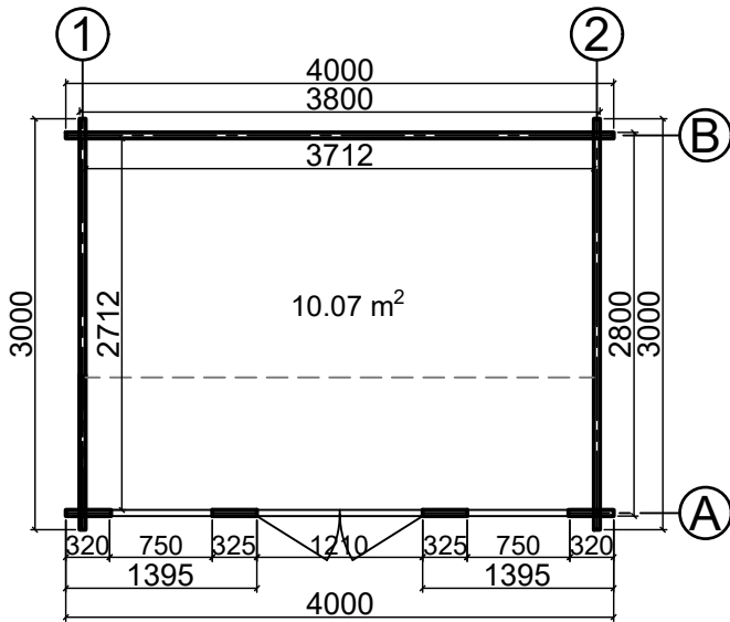
Floor plan
