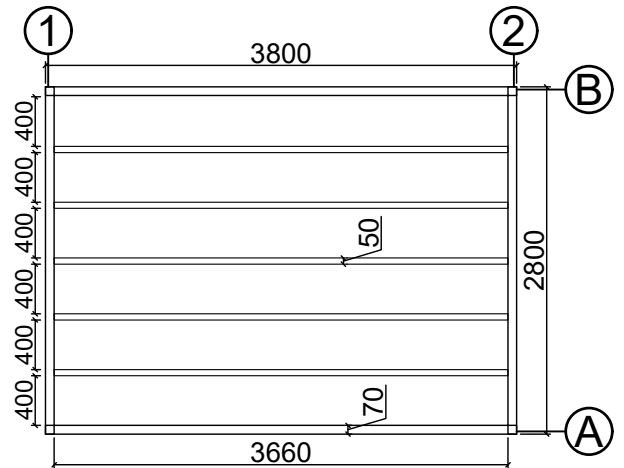
Base plan
