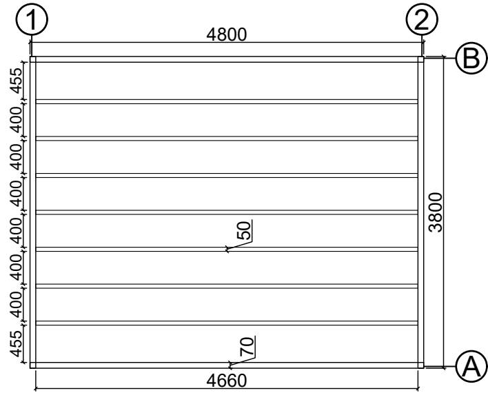
Base plan
