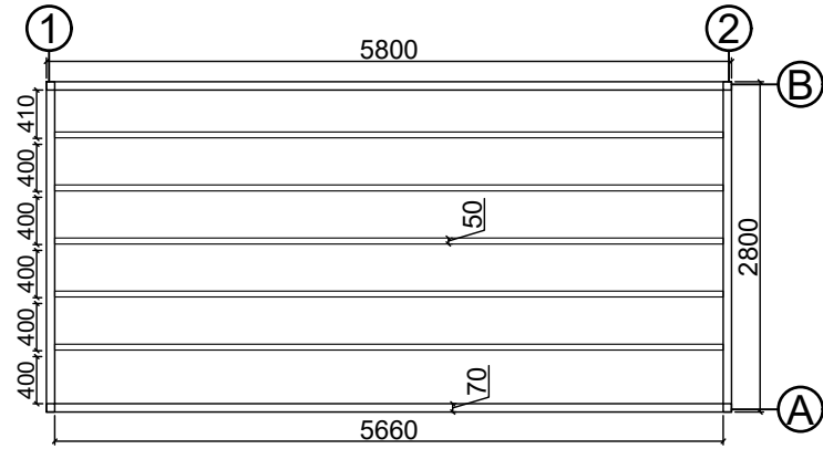
Base plan
