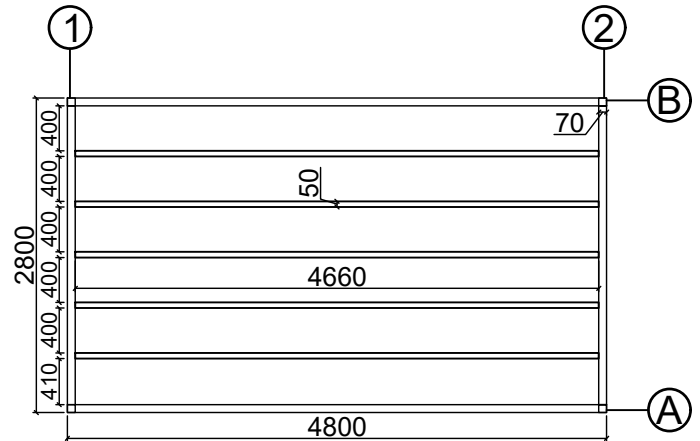
Base plan
