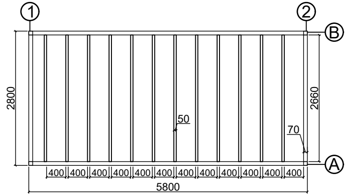
Base plan
