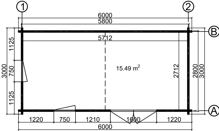
Floor plan
