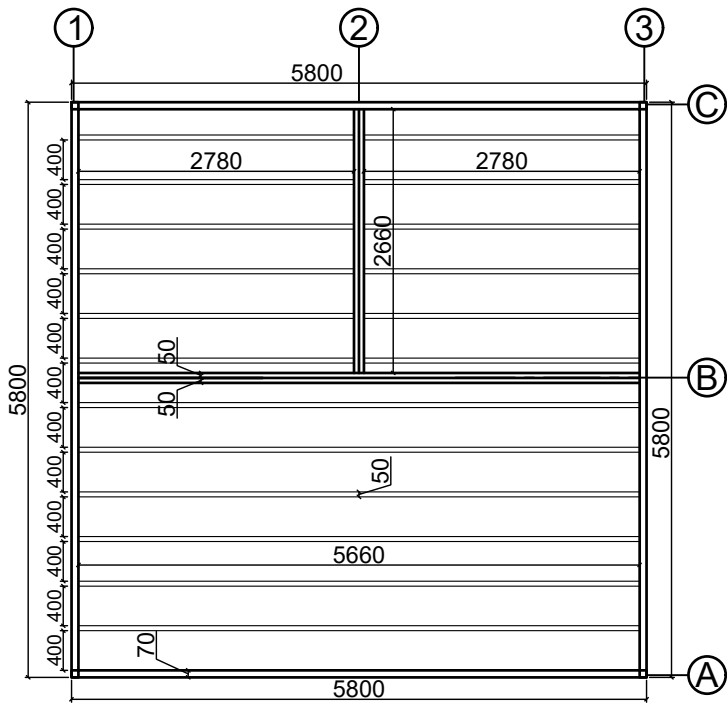
Base plan
