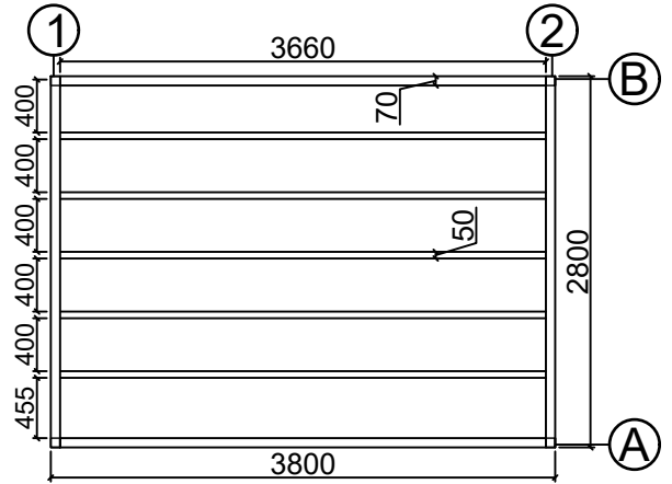
Base plan
