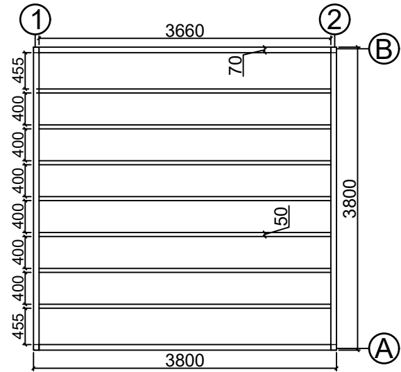
Base plan
