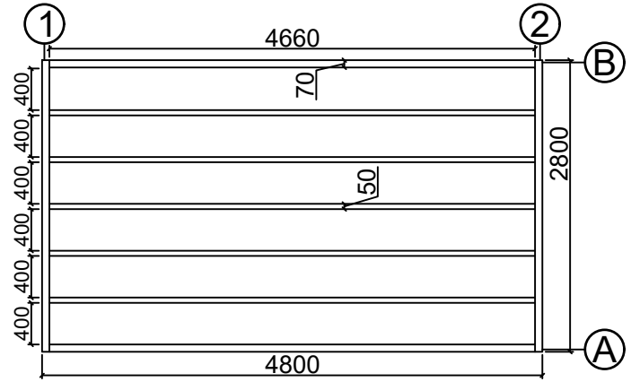
Base plan
