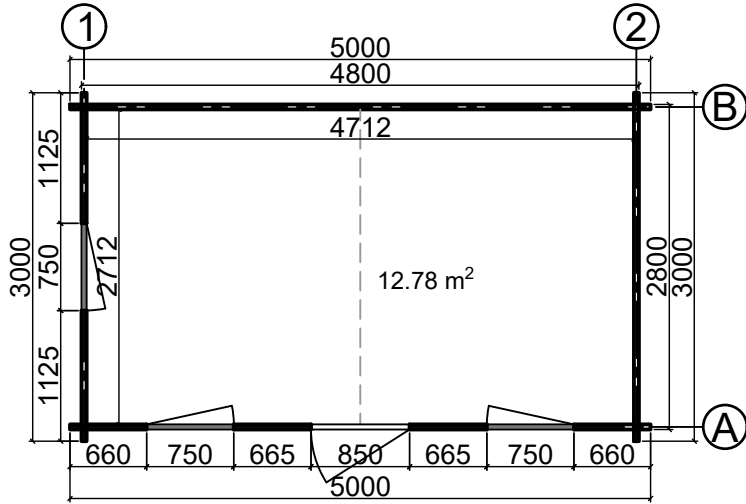
Floor plan
