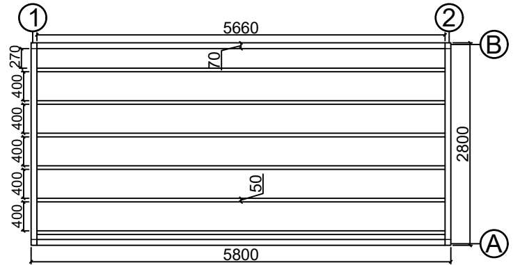
Base plan
