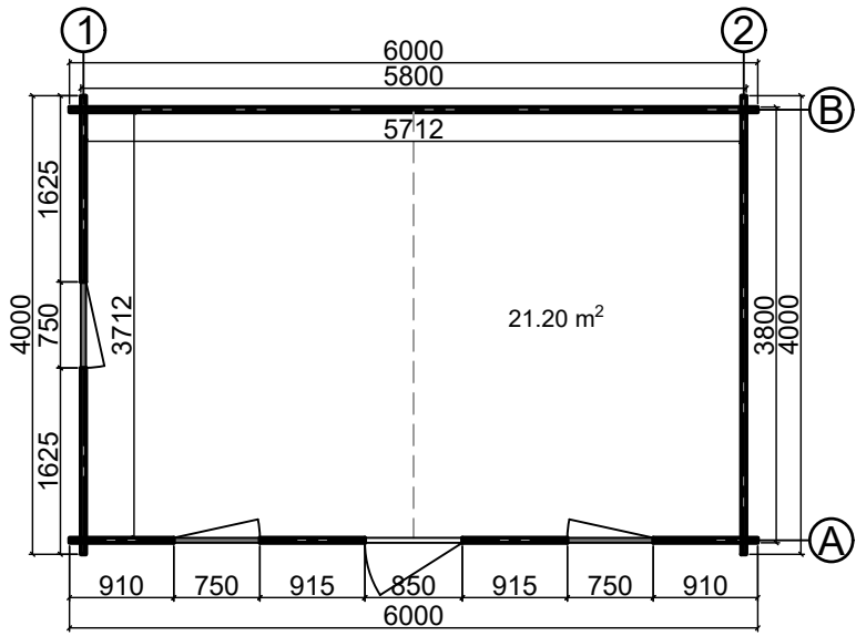
Floor plan
