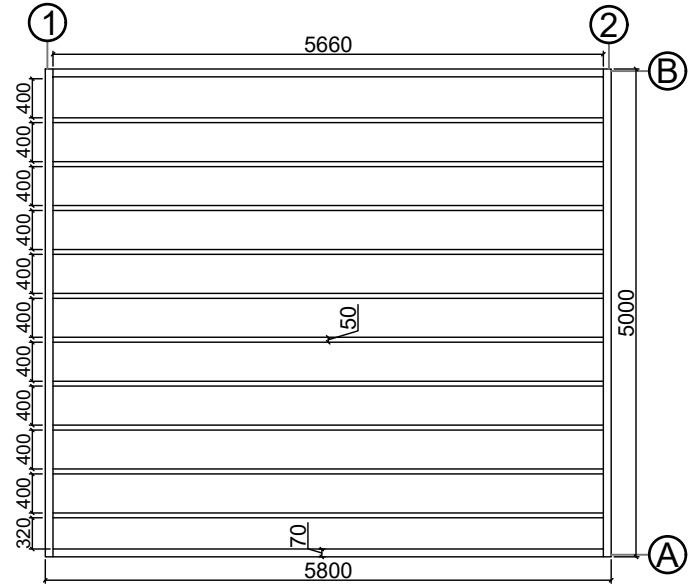
Base plan
