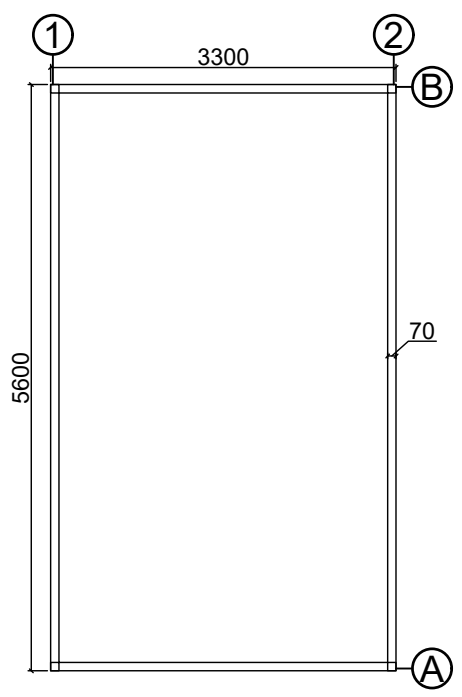
Base plan
