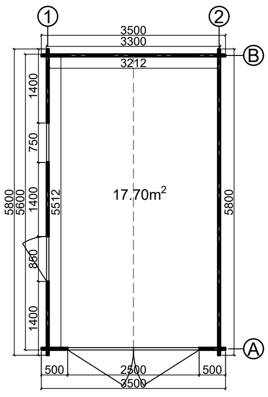
Floor plan
