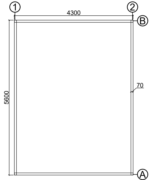
Base plan
