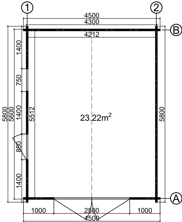
Floor plan
