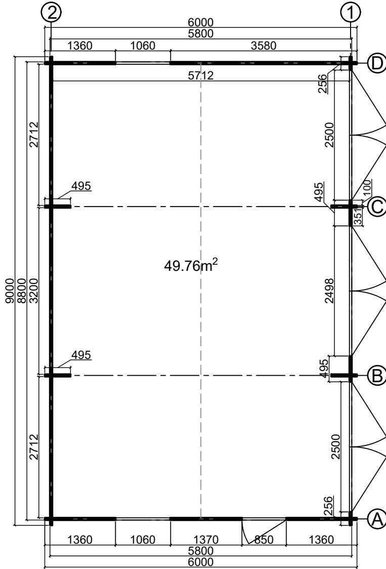
Floor plan
