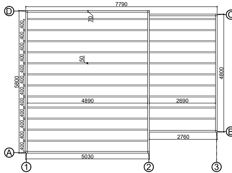
Base plan
