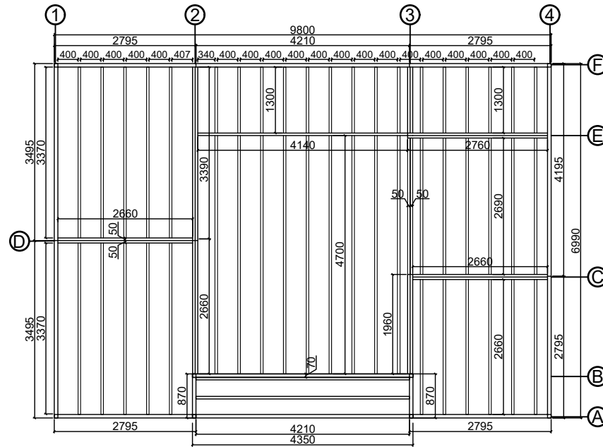
Base plan
