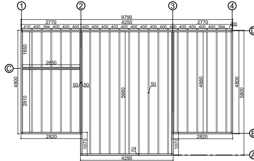
Base plan
