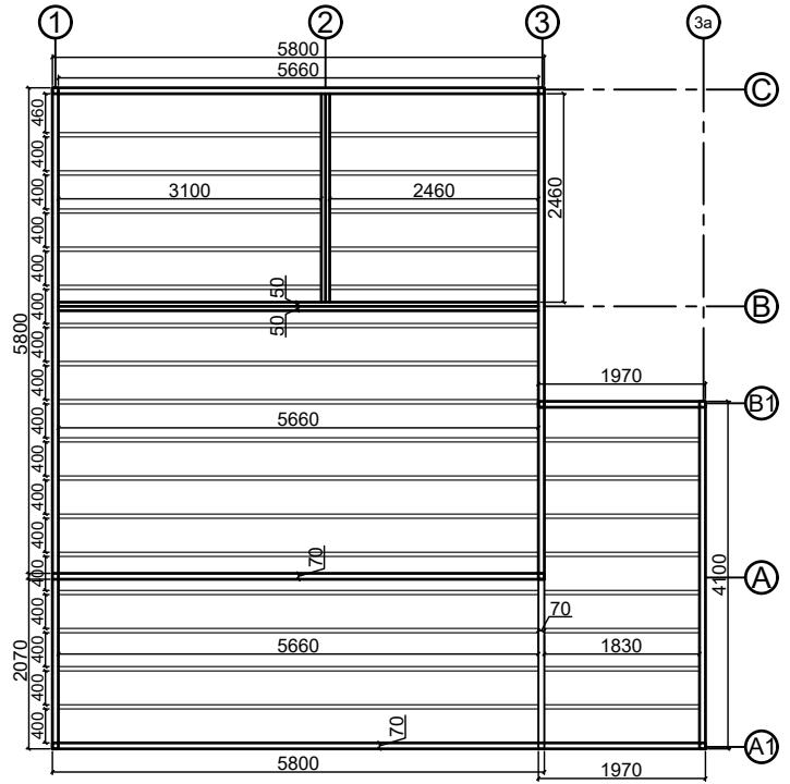
Base plan
