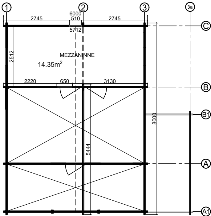
Mezzanine plan
