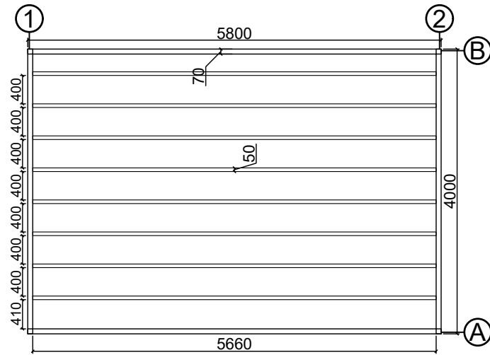
Base plan
